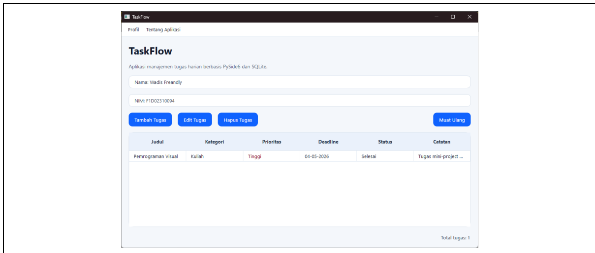
Gambar 4.1 Tampilan Home
